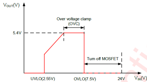
Figure 30 Output vs Input voltage
